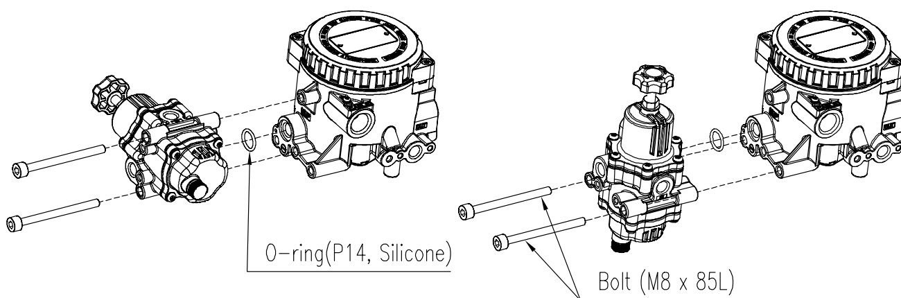
Fig. 2-3: Exploded view
