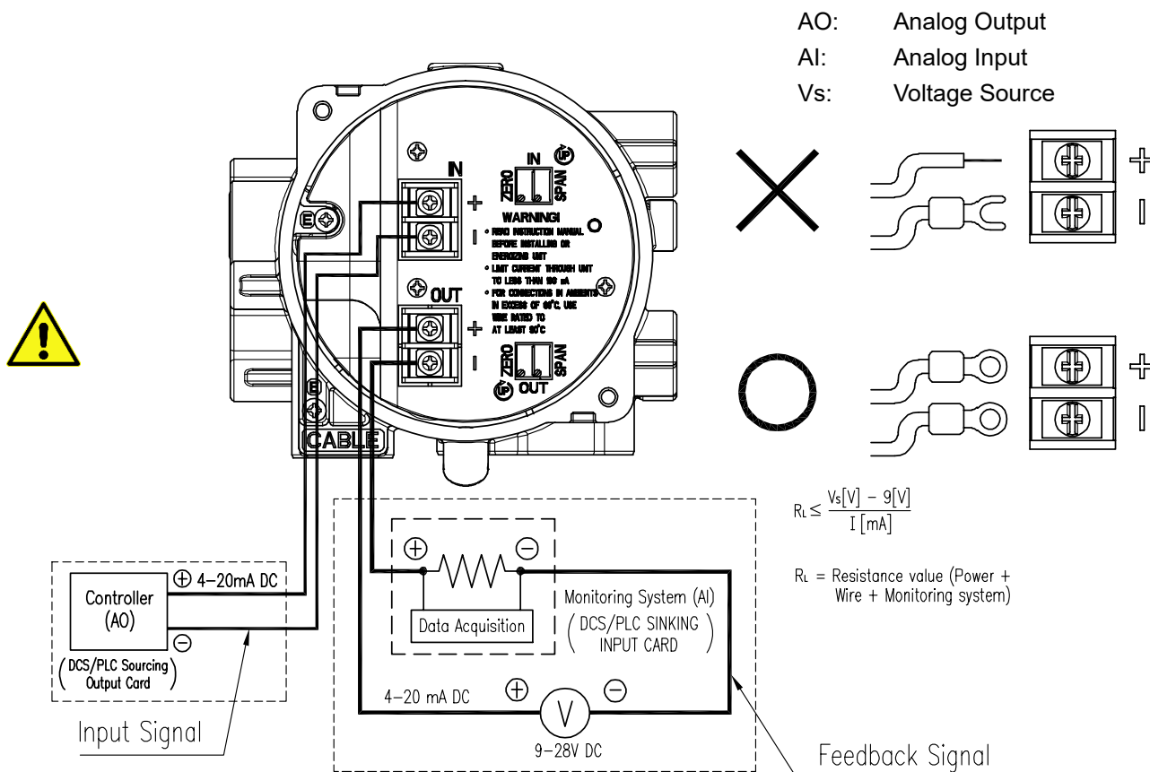
Fig. 5-1 Terminal Overview
