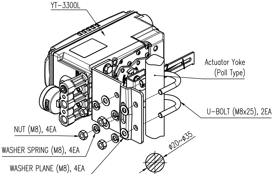
Pole Type Actuator Yoke
