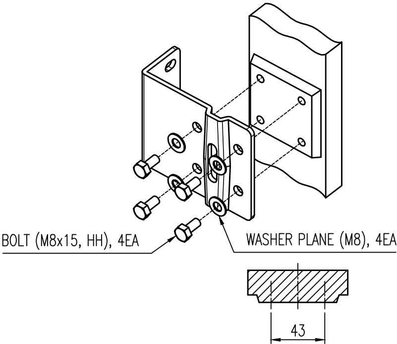
Plane Type Actuator Yoke
