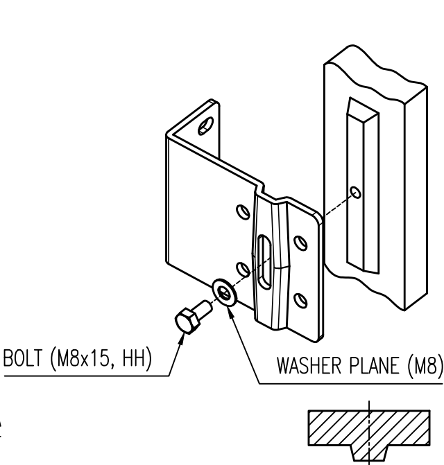
Rib Type Actuator Yoke
