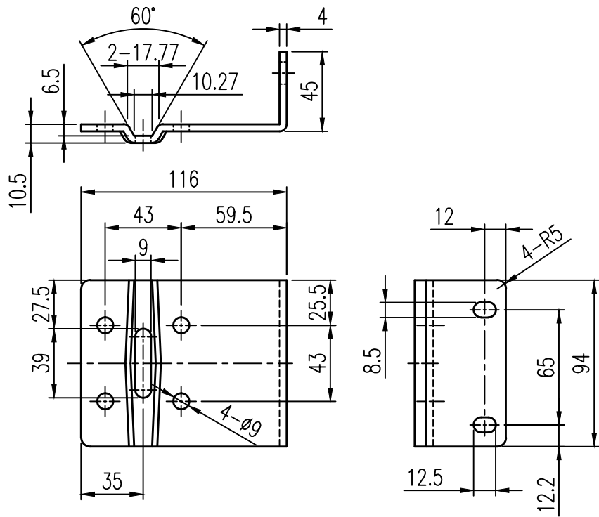
Linear Namur Bracket
