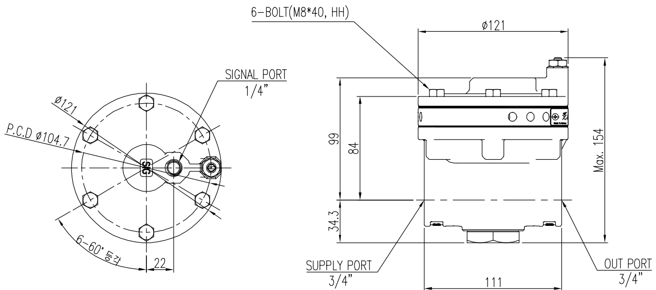
Fig. 2-6: YT-310 / 315 dimension
