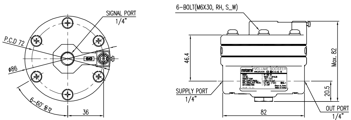
Fig. 2-5: YT-300 / 305 dimension
