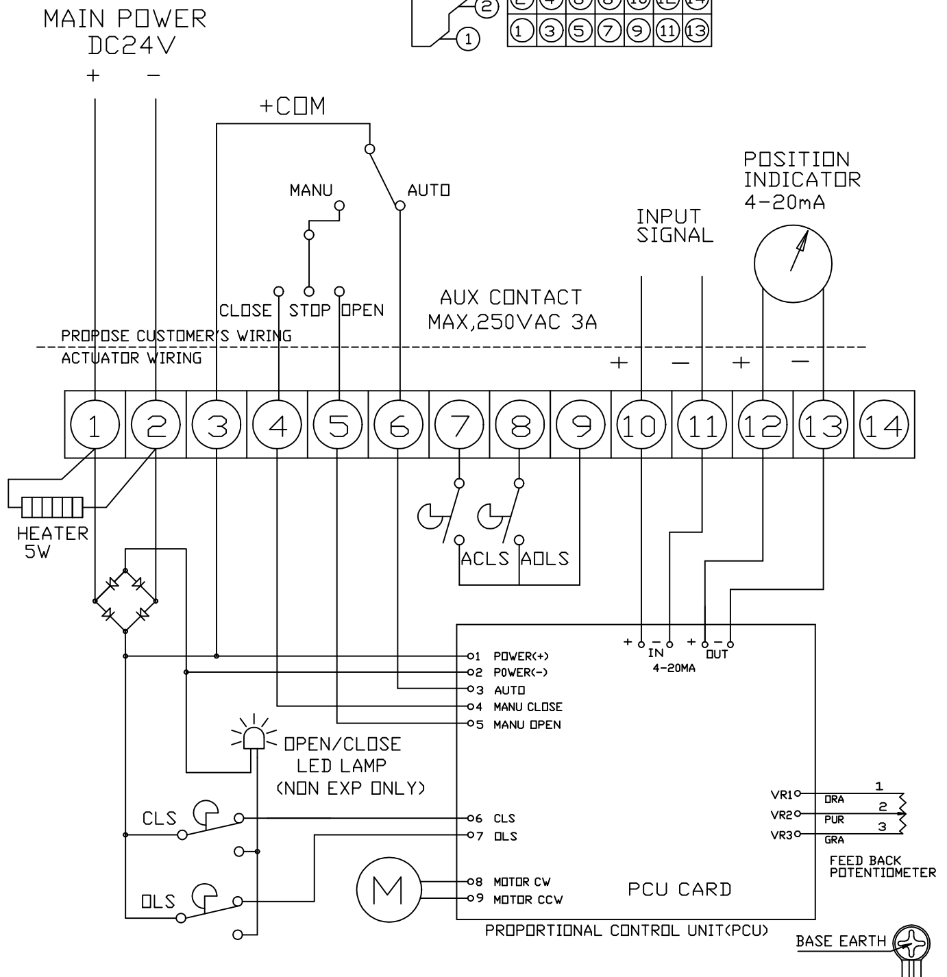
TERMINAL LAYOUT
