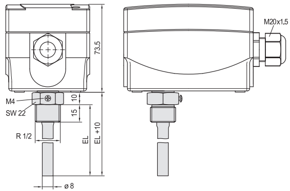
TBT-2G 0/90-U (all measurements in mm)
