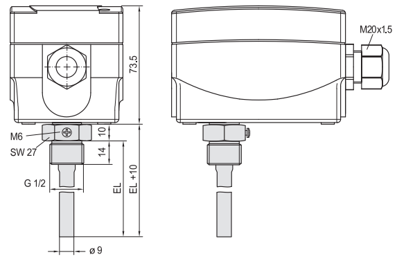
TBT-VA-2G -35/35-U (all measurements in mm)
