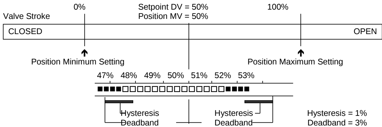
Fig 6: Deadband and Hysteresis settings
