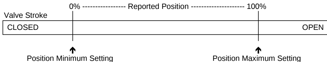
Fig 5: Limited Range Position Control and Reporting
