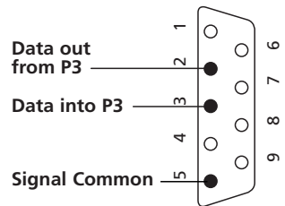
9 way Female D Type RS232 Connections
