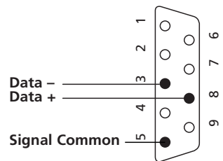
9 way Female D Type RS485 Connections
