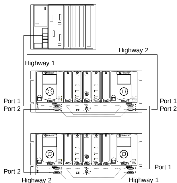
Fig 6: Single Host, dual redundant RS485 comms
