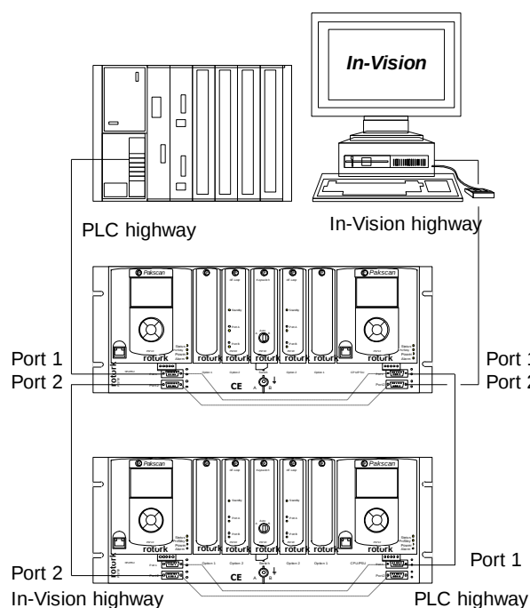
Fig 5: Twin Host, single RS485 comms
