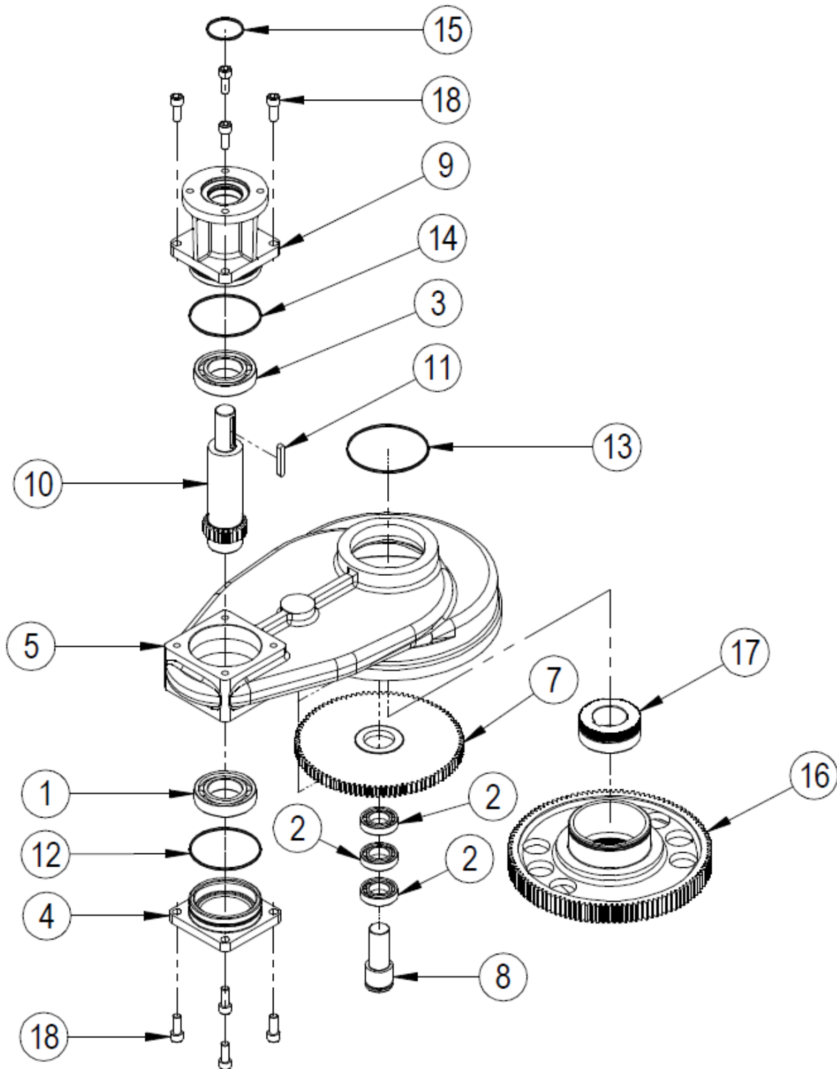
EXPLODED VIEW FOR AS INPUT REDUCER
