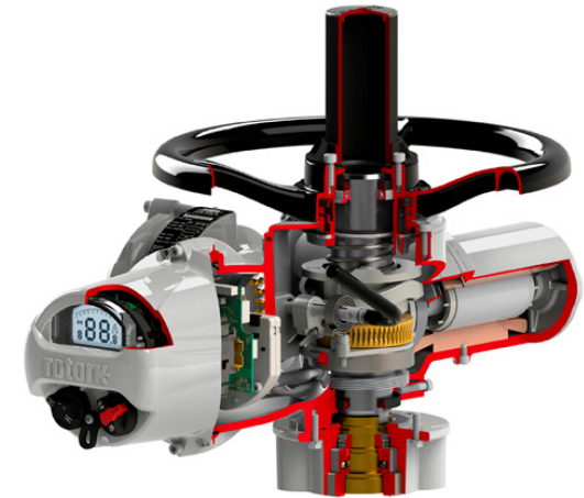
Above: Cutaway drawing of the Rotork IQ3 non-intrusive, intelligent electric valve actuator.
