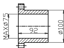
BASE&DRIVE BUSHING
