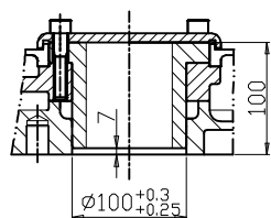
BASE&DRIVE BUSHING
