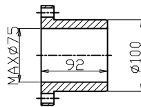
BASE&DRIVE BUSHING
