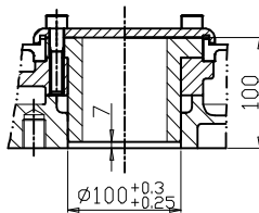
BASE&DRIVE BUSHING
