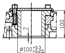
BASE&DRIVE BUSHING
