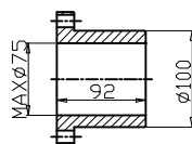
BASE&DRIVE BUSHING
