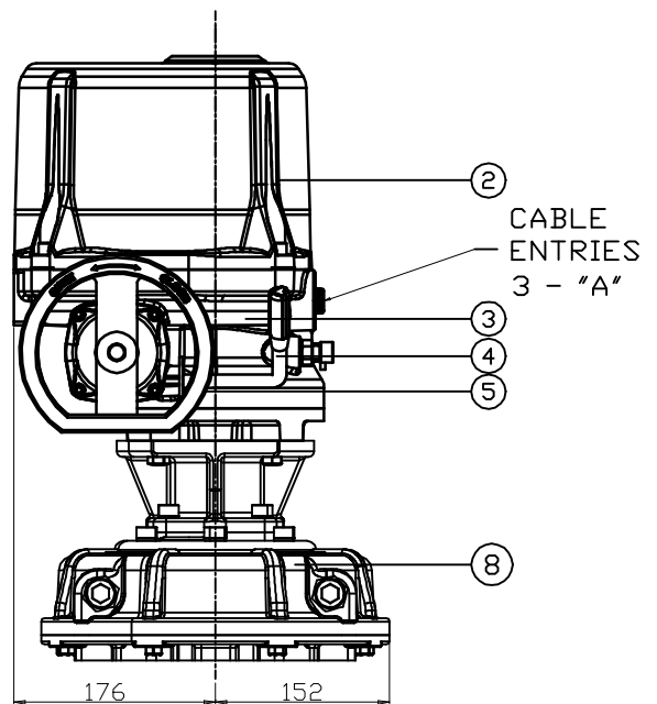
BASE
