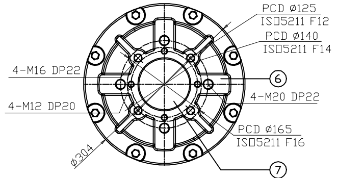
BASE
