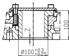
BASE&DRIVE BUSHING
