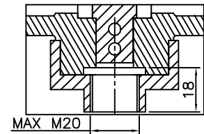
BUSHING
