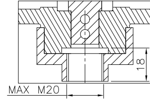
BUSHING
