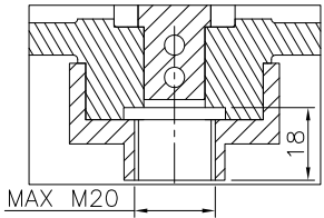
BUSHING
