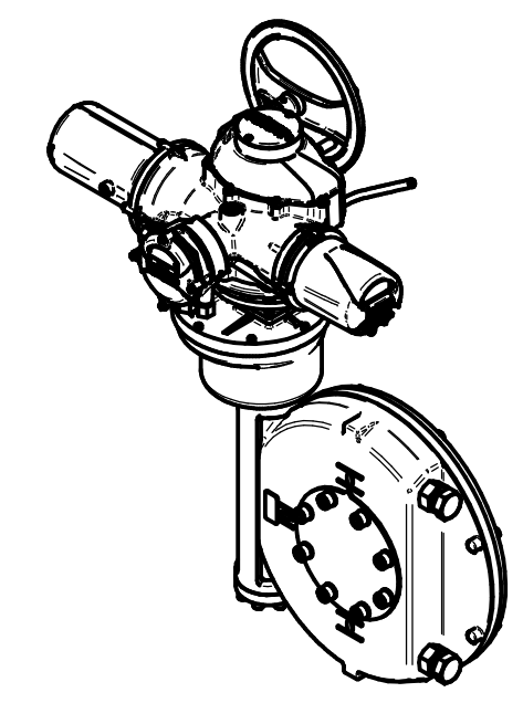
ISOMETRIC VIEW (SCALE 1:20)
