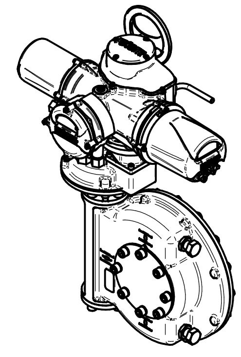
ISOMETRIC VIEW (SCALE 1:12)
