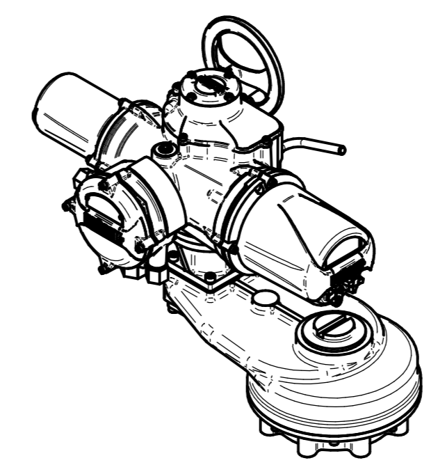
ISOMETRIC VIEW 1:10
