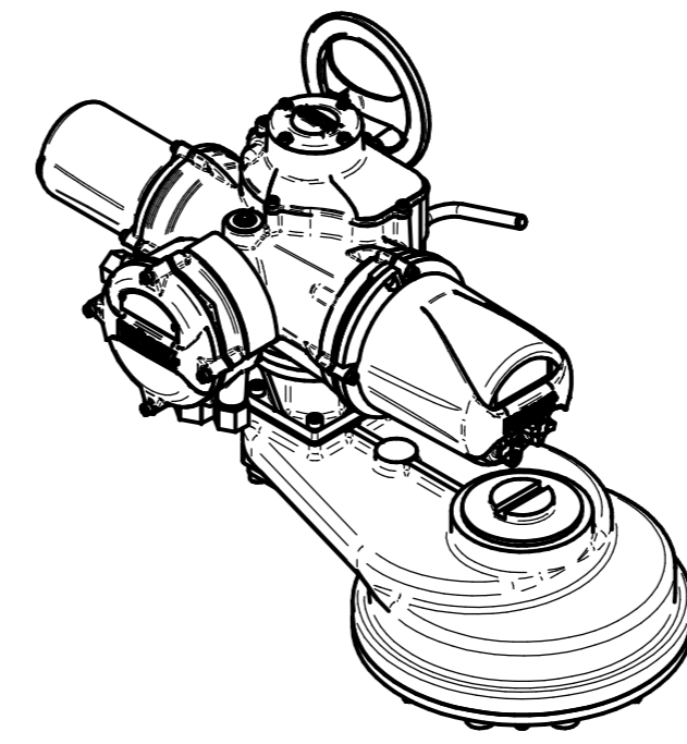
ISOMETRIC VIEW 1:10
