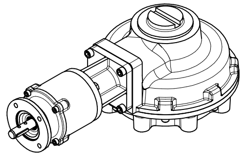
E-FLANGE INPUT ISOMETRIC VIEW 1:8
