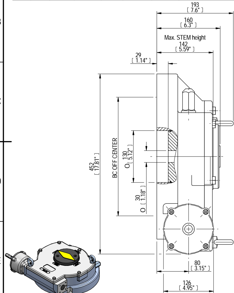
ISOMETRIC VIEW 1:10
