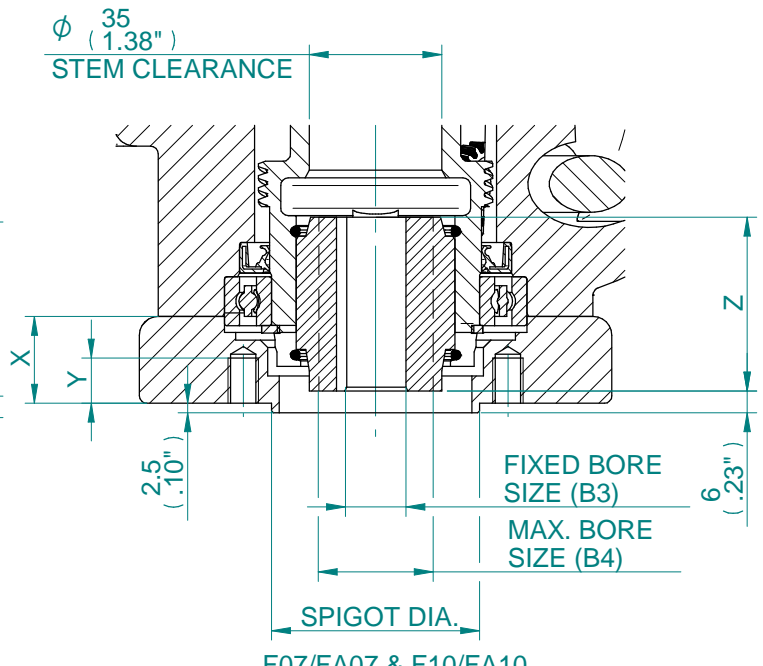
F07/FA07 & F10/FA10 TYPE "B3 & B4" COUPLING DETAILS
