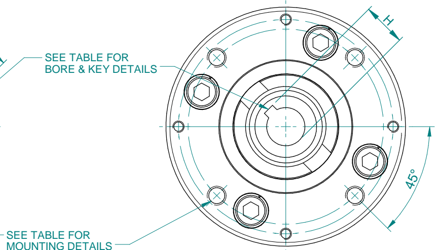
F07/FA07 & F10/FA10 NON THRUST BASE (B3 & B4)
