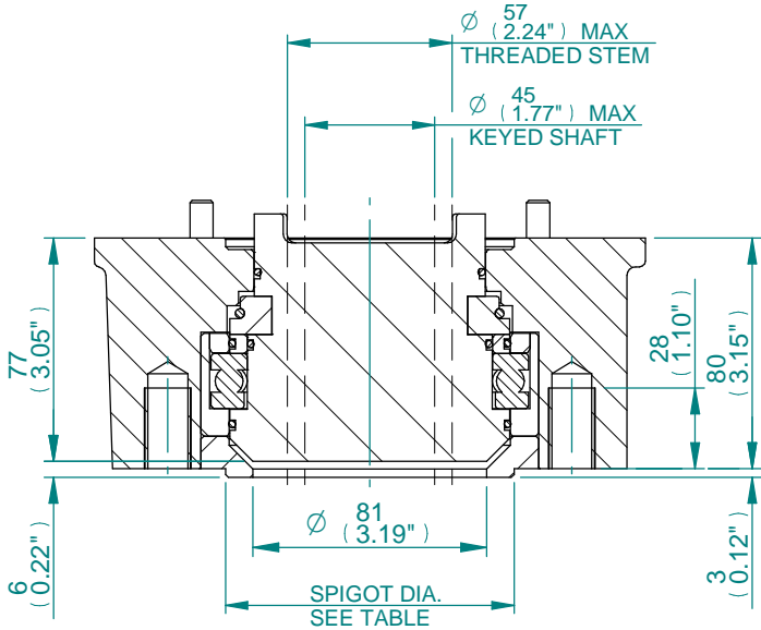
TYPE "A" COUPLING DETAILS
