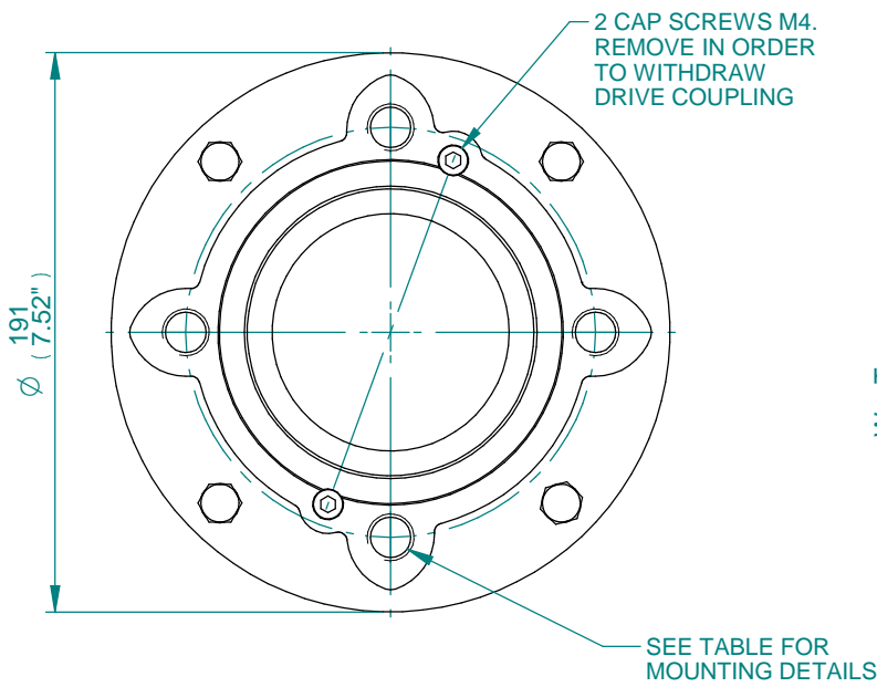
F14/FA14 THRUST BASE
