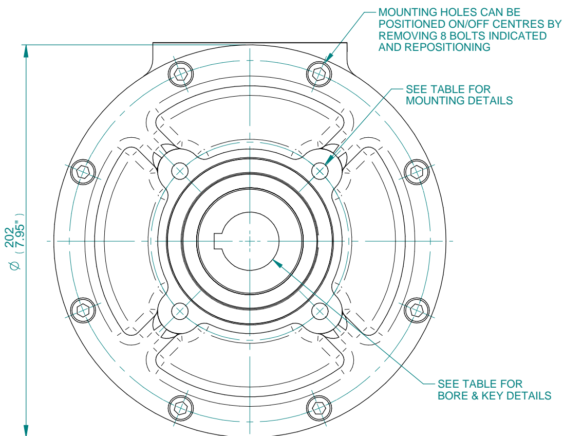
IB4 GEARBOX MOUNTING DETAILS
