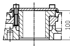
DRIVE BUSHING
