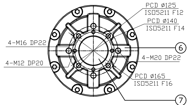
BASE
