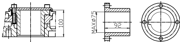
DRIVE BUSHING
