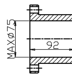
DRIVE BUSHING
