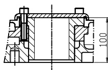
DRIVE BUSHING
