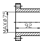
DRIVE BUSHING
