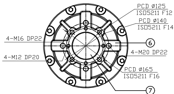
BASE
