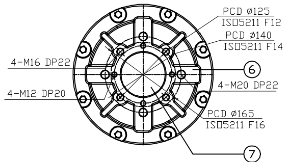
BASE
