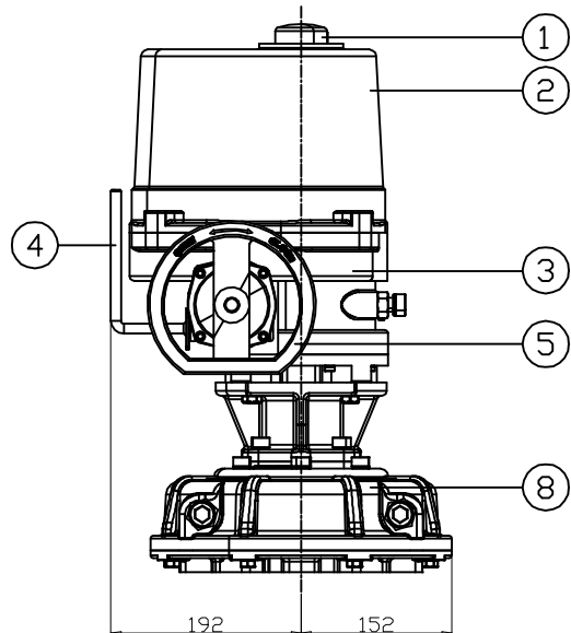
BASE
