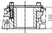
DRIVE BUSHING
