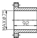
DRIVE BUSHING
