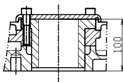
DRIVE BUSHING
