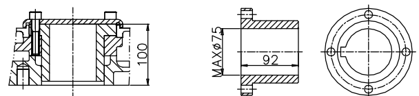
DRIVE BUSHING
