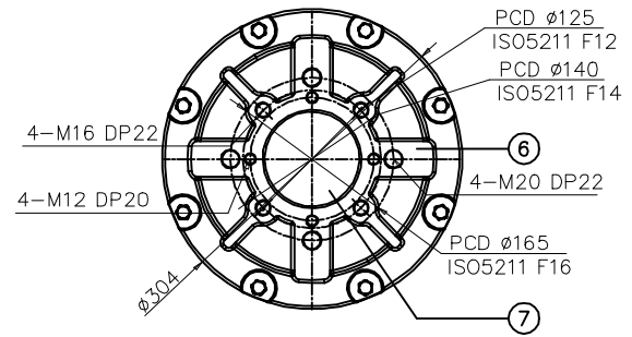
BASE
