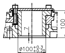
BASE&DRIVE BUSHING
