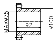
BASE&DRIVE BUSHING
