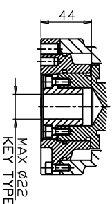
BASE & D/B
